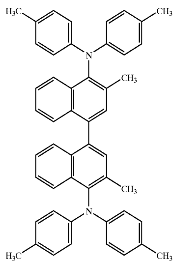
Compound described in JP-A 11-152253
